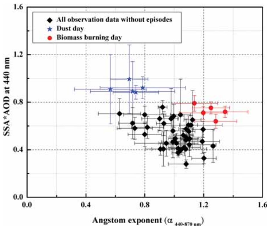
Fig. 10. Scatterplot of daily-averaged Ångström exponent and scattering coefficient (AOD · SSA at 440 nm) in the observation period over Shanghai. The averages with standard deviation were calculated from all inversed AOD, SSA and Ångström exponent in each observation day. Five samples were for dust (in blue) and five samples were for biomass (in red) while forty samples represented normal condition (in black).
