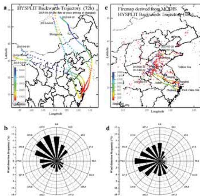
Fig. 3. Backward trajectories based on HYSPLIT model and firemaps derived from MODIS with wind roses during observation period. (a) Hourly resolved 72 h air mass back trajectories during dust episodes (five days); (b) wind roses during five dust days using hourly-averaged data for analysis; (c) hourly resolved 48 h air mass trajectory with daily firepots derived from MODIS during biomass burning episode (five days); (d) Wind roses during five biomass burning days using hourly-averaged data for analysis.
