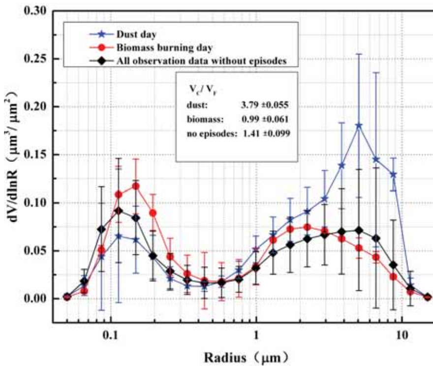
Fig. 7. Average aerosol volume size distribution with standard deviation in the observation period over Shanghai. The averages and deviations were calculated from each inversed volume concentration in 22 radius during five dust days (in blue), five biomass burning days (in red) and forty normal days (in black).
